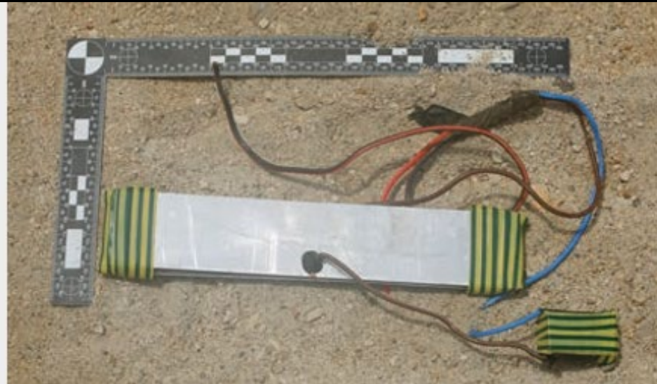
Improvised pressure-plates
